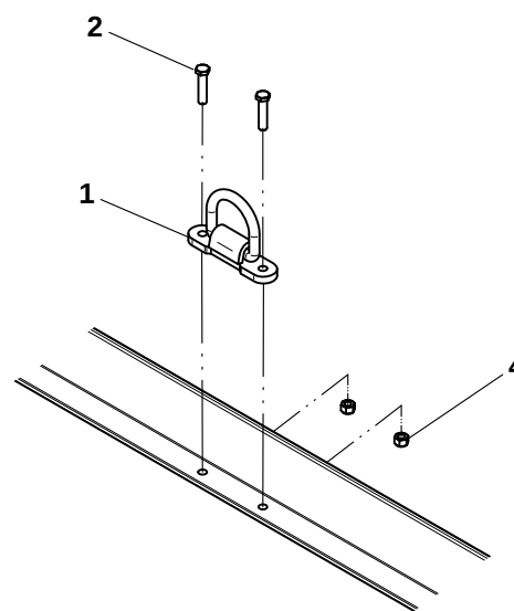
STEEL DECK
