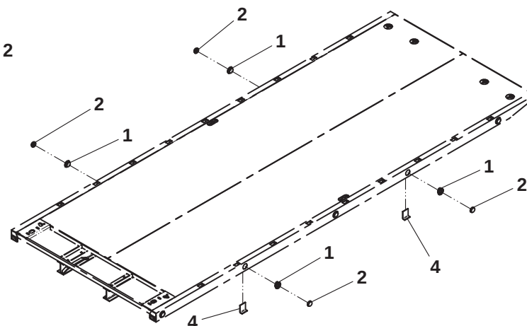
STEEL DECK
