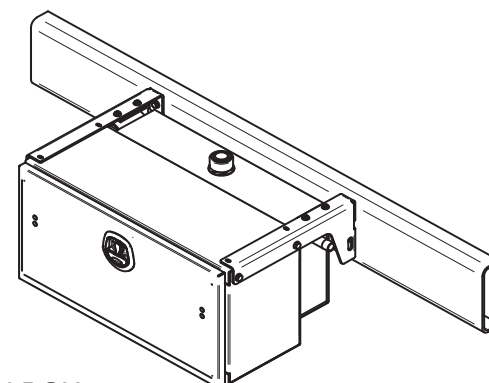
36" TOOLBOX w/ HYDRAULIC RESERVOIR
